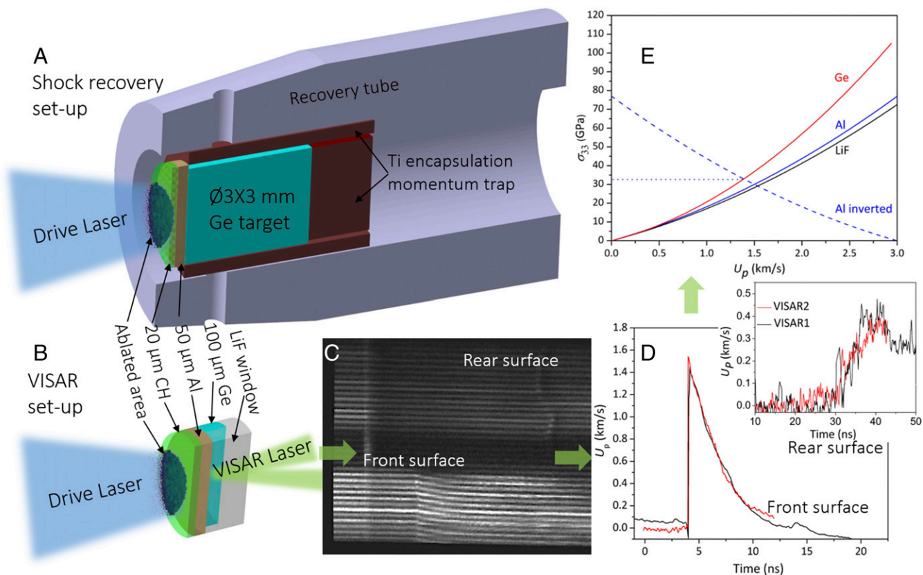
Fig. 1. Laser-driven, shock-recovery experimental setup, velocimetry measurement, and determination of shock stresses. (A) Shock-recovery assembly with target package (along the laser path: 20- \mu\text{m} CH ablator, 50- \mu\text{m} Al pusher, and \text{Ø}3 \times 3\text{-mm} Ge crystal) encapsulated in Ti and backed by momentum trap (Ti). The assembly is mounted in a recovery tube. (B) VISAR target package is similar to that of the recovery experiment except that a 100- \mu\text{m} -thick half-cylindrical Ge foil is used so as to capture the information from both front (Al/LiF) and rear (Ge/LiF) surface of the target. The laser-transparent LiF window is glued to the rear surfaces of Ge target on one side and Al pusher on another side. (C) Temporally resolved VISAR fringes showing the shock breakout at front and rear surfaces of the sample. (D) Measured particle velocity, U_p as a function of time. (E) Determination of the peak shock stress on the front surface of Ge target by impedance matching. Note that Al and LiF are closely impedance-matched in the regime involved in our study.
